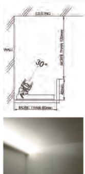
30 degrees adjustable
