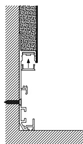
Step 04 Stick the led strip and snap the cover
