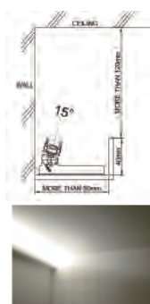
15 degrees adjustable
