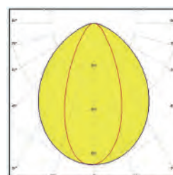
Lens 55°
