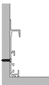
Step 01 Fix the Aluminum base first
