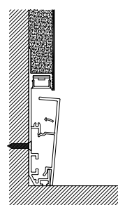
Step 05 Install the adjustable aluminum cover
