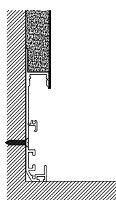
Step 03 Paint the drywall
